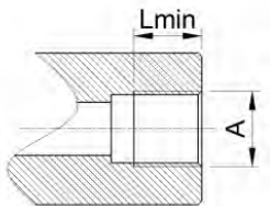
依据锥形英制管螺纹 (BSPT螺纹)
